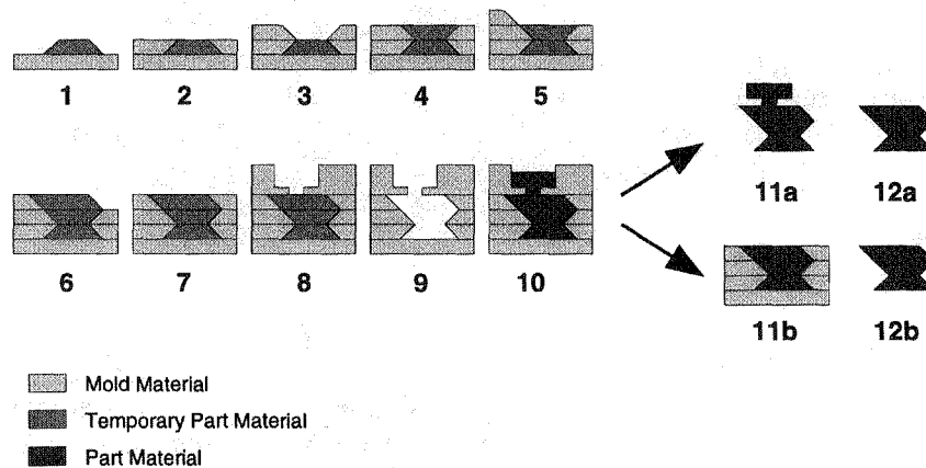
Figure 1: Example Mold SDM process sequence
