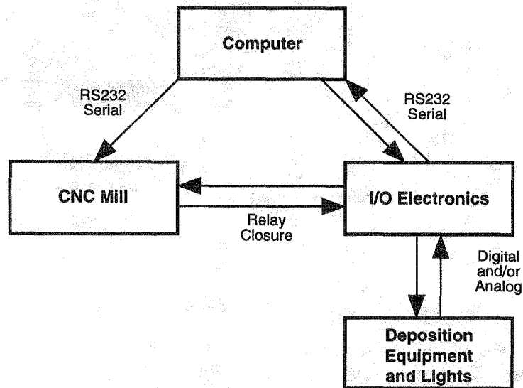
Figure 4: Machine control schematic
