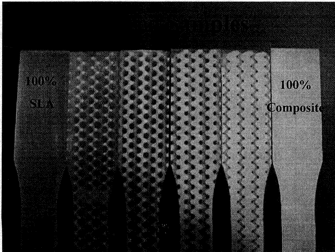
Figure 6. Sliced Samples
