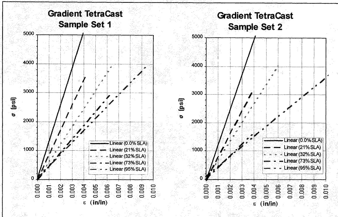
Figure 7. Stress Strain Curves for Gradient Tetracast Samples
