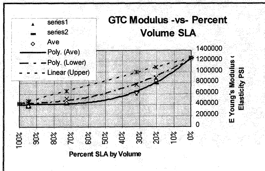
Figure 8. Modulus as a Function of Composition
