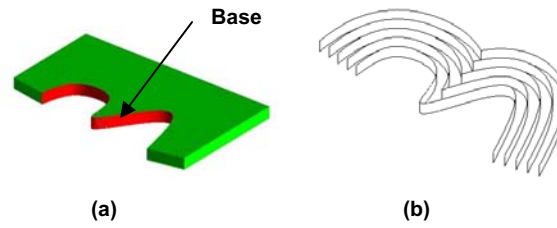
Figure 4: Non-planar slices – offsets of the base surface
