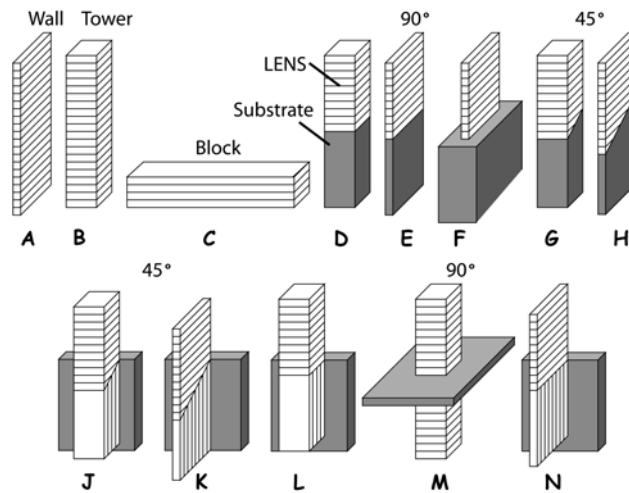
Figure 4. Schematic of 13 Different Types of LENS Deposited Tensile Test Specimen Representing Repair and Modification Geometries.
