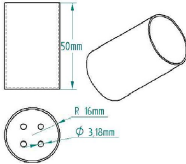
Figure 2: Canister part with vent holes and no taper.
