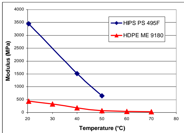
Figure 1: Elastic modulus at various temperatures for HDPE and HIPS.
