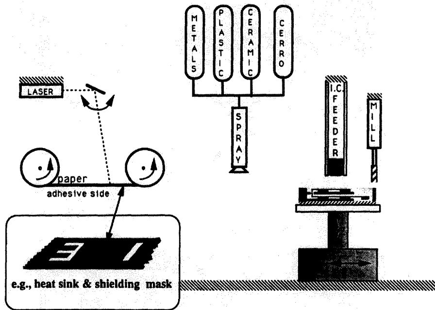
Figure 2: MD* System Configuration.
