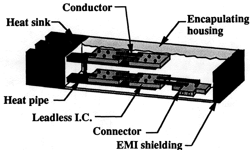
Figure 4: Integrated electronic/mechanical package.
