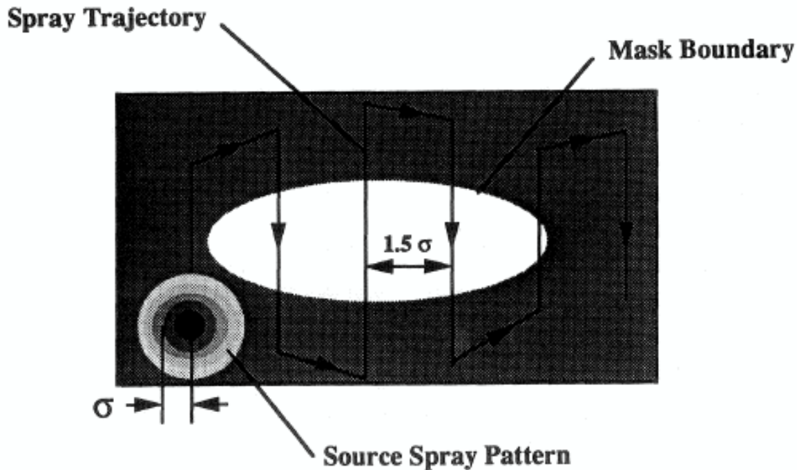
Figure 1: Spray trajectory.
