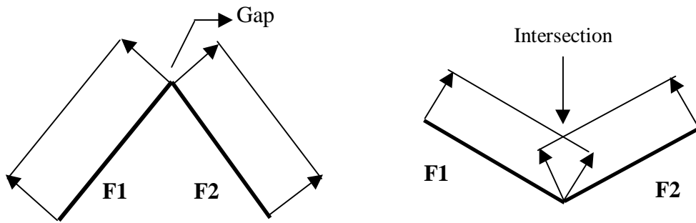
Figure 2a. Gap between offset surfaces Figure 2b. Intersection between offset surfaces
