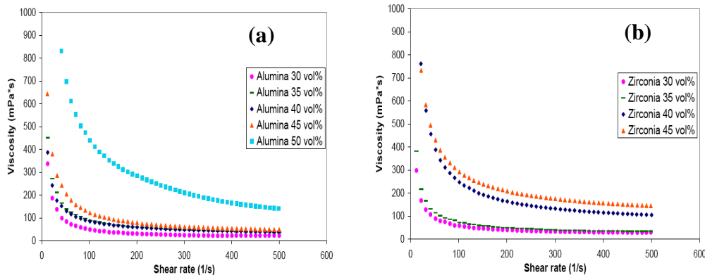
Fig.2 Flow curve (viscosity vs. shear rate) of alumina (a) and zirconia (b) slurries showing the effect of the increase in solid loading on the viscosity
