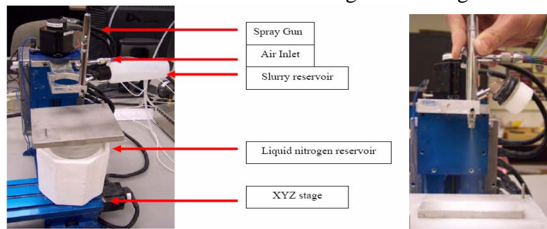
Figure 1. Experimental apparatus showing a system employed for sample fabrication process
