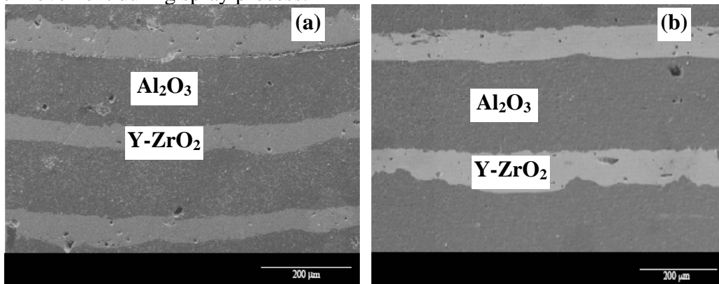
Figures 4a and 4b. SEM micrographs of alumina/zirconia samples, showing uniform layer geometry
