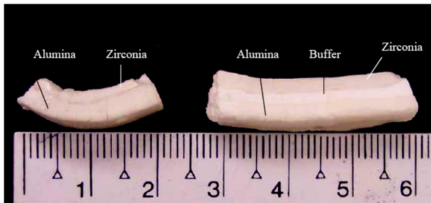
Figure 6. An alumina/zirconia composite (left) and an alumina/buffer/zirconia composite (right)
