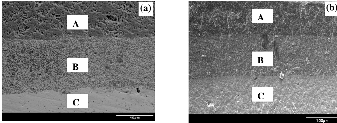
Fig. 5 SEM micrographs showing a cross sectional view of a polished (a) and unpolished (b) alumina/buffer (50 vol% alumina + 50 vol% zirconia)/zirconia composite
