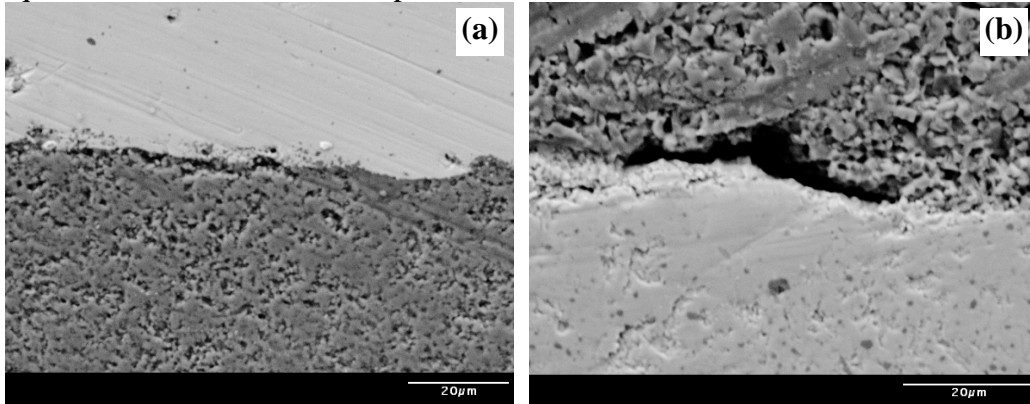
Fig. 7 SEM micrographs showing cracks and voids along the interfaces of the alumina and zirconia layer
