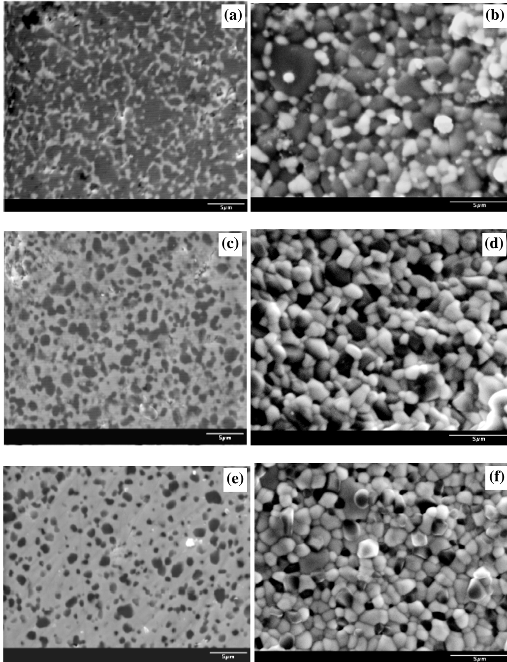
Fig. 9 SEM micrographs of buffer layers with 80% alumina / 20% zirconia (a-b), 60% alumina / 40% zirconia (c-d), and 20% alumina / 80% zirconia (e-f),
