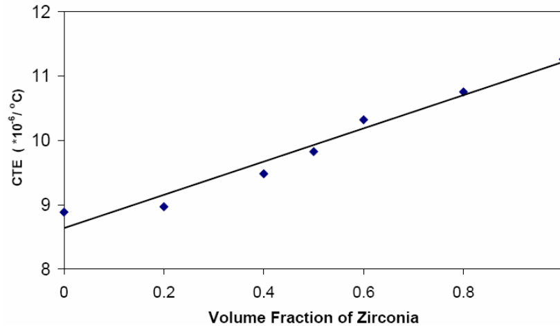
Fig.10 Coefficient of thermal expansion of samples as a function of zirconia volume fraction
