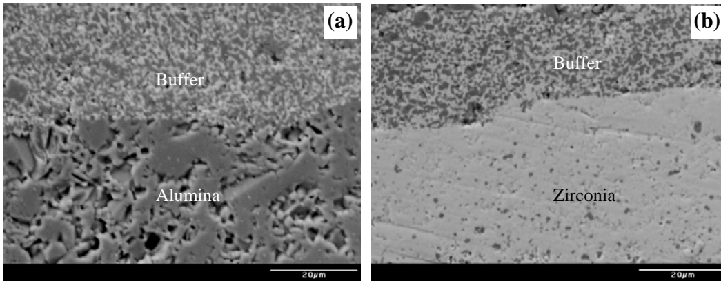
Fig. 8 SEM micrographs showing interfaces between buffer/alumina (a) and buffer/zirconia (b) layer
