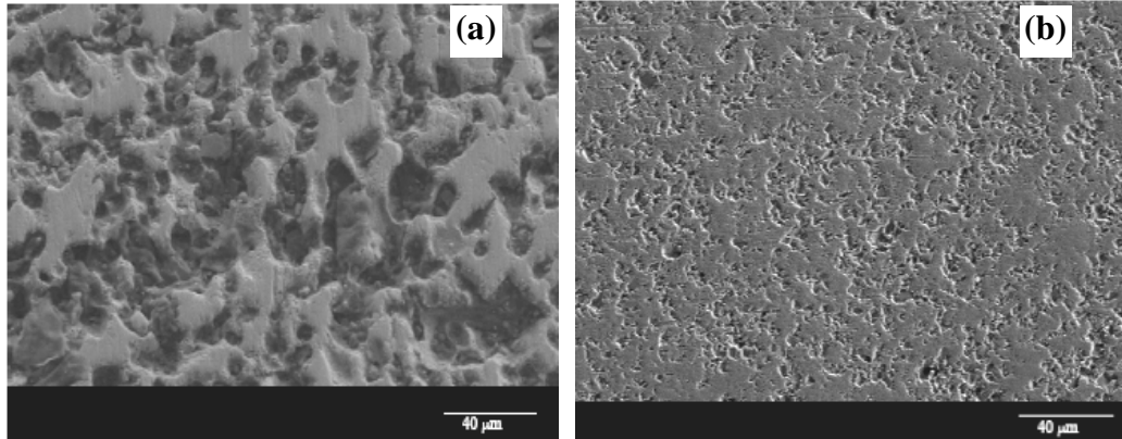
Fig.3 SEM micrograph of microstructure of alumina in an un-press (a) and isostatically-pressed (b) sample
