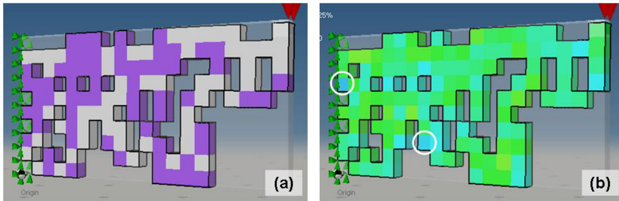
Figure 5 – Cantilever Beam Results From DesignLab for Two Materials, Showing Material Distribution Plot (a) and Stress Distribution Plot (b) with Areas of Localised Stress Circled
