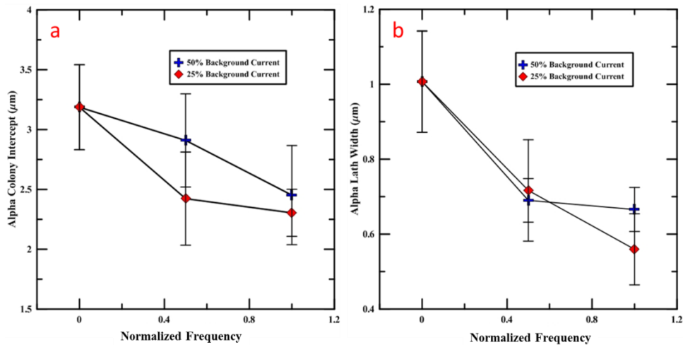
Figure 13 \alpha colony intercept lengths (a) and \alpha lath width (b) for both modulated conditions. Largest refinement and smallest lath spacing occurs for the deposition conditions for deposit 5 in Table 1.
