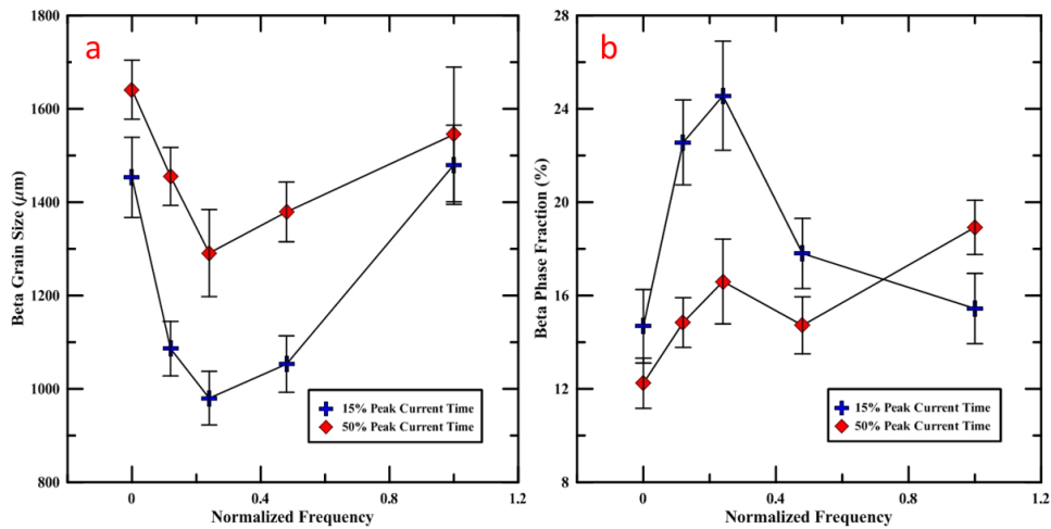
Figure 18 \beta phase refinement due to arc modulation: (a) \beta grain size for both modulation conditions; (b) \beta phase volume fraction increase for both waveform conditions.
