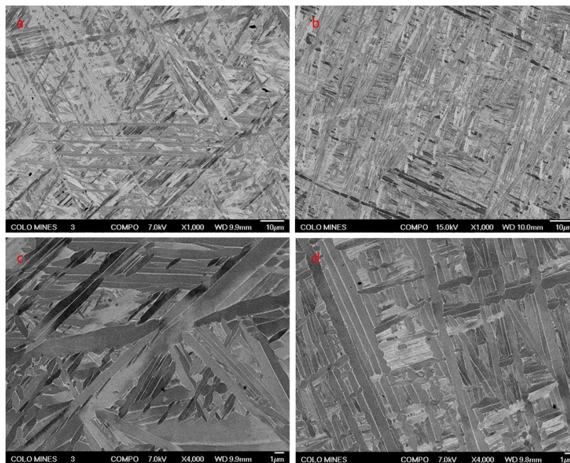
Figure 20 Refinement of \alpha phase due to arc modulation: (a) Baseline build with no modulation at low magnification; (b) Modulated build at low magnification; (c) Baseline build with no modulation at high magnification; (d) Modulated build at high magnification.
