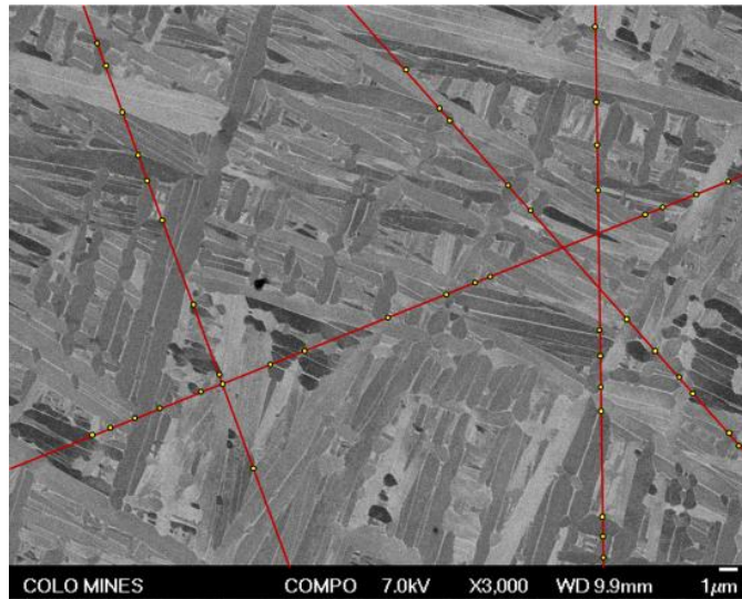
Figure 7 Colony intercept length is determined by the placement of random line segments of known length. At the intersection of two colonies, notice the placement of a yellow dot. The number of the intercepts, yellow dots, per unit line length can be used to find average colony intercept length.
