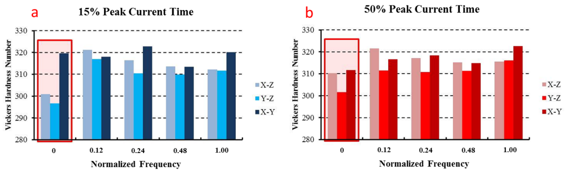
Figure 23 Bar plot showing the hardness in each direction with non-modulated builds highlighted by the red boxes. Hardness was increased by arc modulation in all directions, resulting in a
