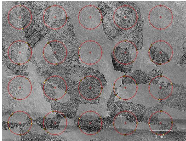
Figure 5 The \beta grain size quantification method of circular intercept. Yellow dots represent intersections with \beta grain boundaries.
