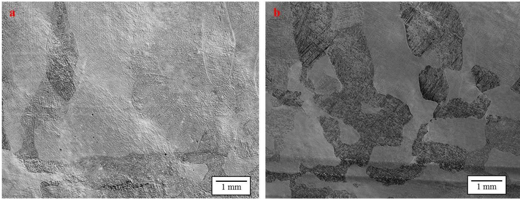
Figure 17 \beta grain refinement due to arc modulation: (a) Non-modulated build macrostructure; (b) Modulated arc macrostructure as described for deposition 8 in Table 2.
