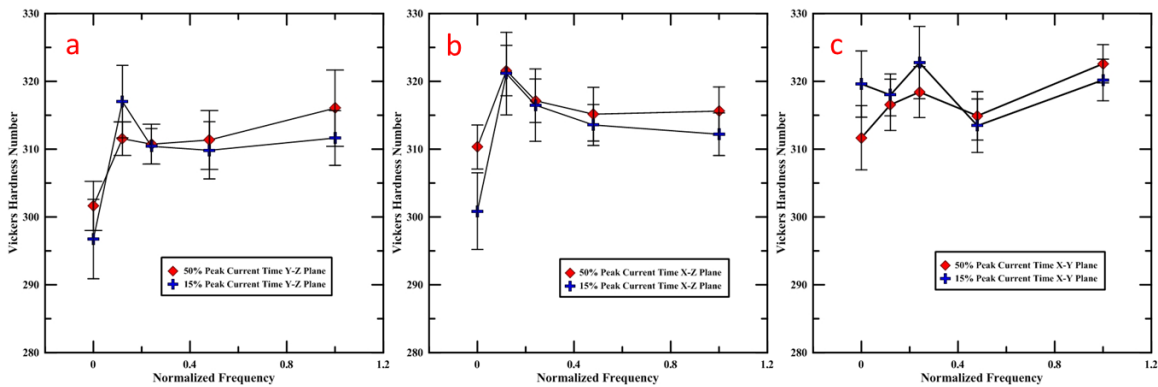
Figure 22 Variation in microhardness with frequency measure in: (a) Y-Z plane; (b) X-Z plane; (c) X-Y plane.
