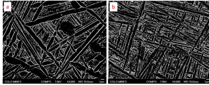
Figure 19 Representative change in \beta phase fraction with arc modulation: (a) Non-modulated builds parameters; (b) Modulated arc build as described for deposit 8 in Table 2.
