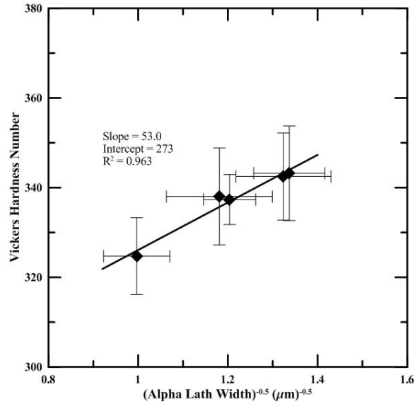
Figure 16 Hall-Petch relationship utilizing \alpha width. The regression coefficient of 0.96 indicates a strong linearity of the data.
