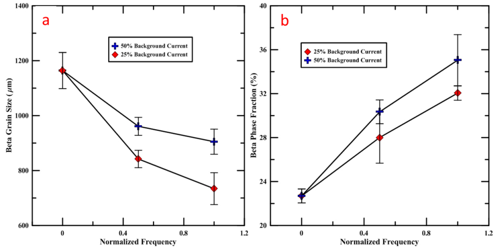
Figure 10 \beta grain size: (a) refinement using modulation for each waveform condition. The largest grain size refinement was observed at maximum modulation frequency. \beta phase volume fraction: (b) was increased from 22.7% to 35.0%.
