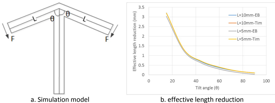
Fig.8 Effective length reduction simulation
