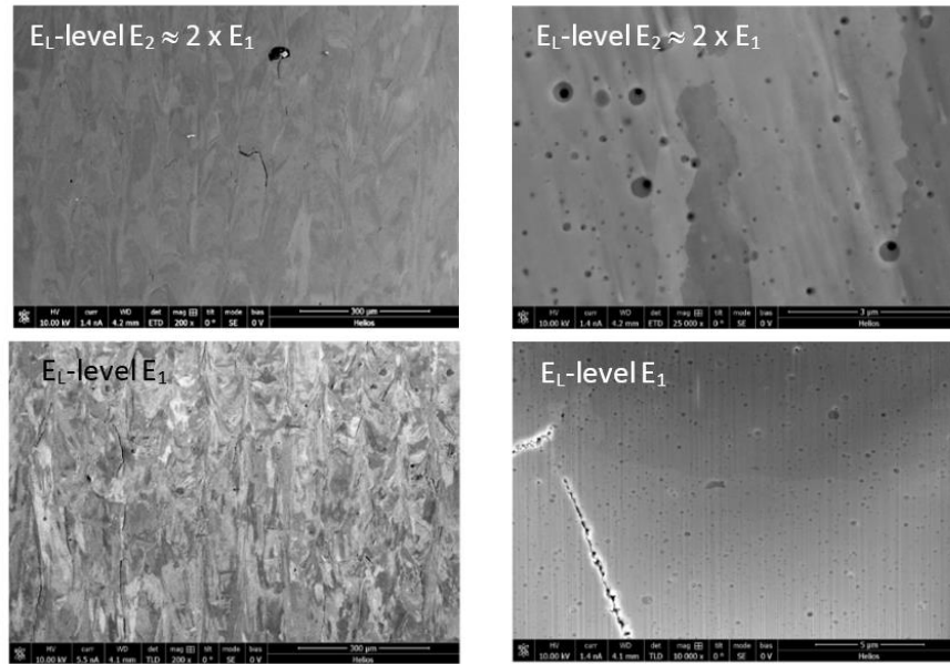
Figure 5: Microstructural analysis of IN625-ODS. Bottom: Energy level E_1 , Top: Energy level E_2 \approx 2 \times E_1
