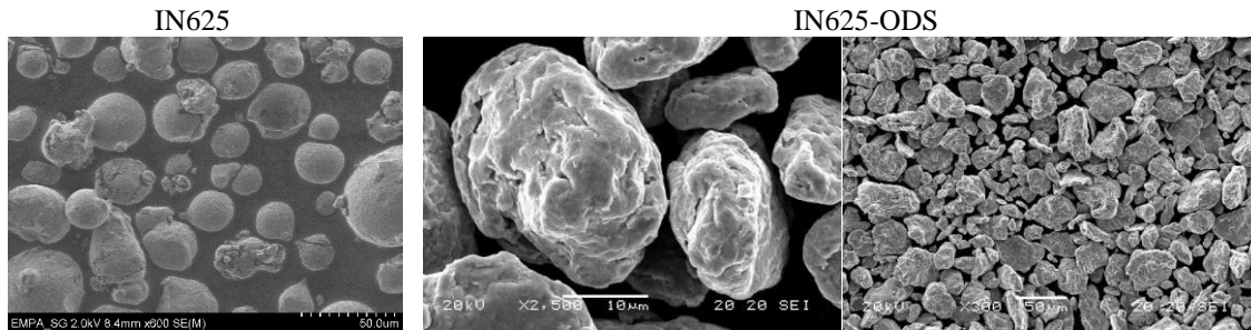
Figure 2: Powder particles for IN625- (left) and IN625-ODS powder (middle and right)
