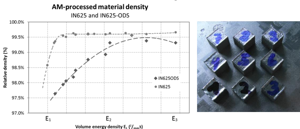
Figure 3: Left: Material density of SLM-processed IN625 and IN625-ODS over volume energy density between E_1 and E_3 ; SLM IN625-ODS samples built on a steel base plate (right).
