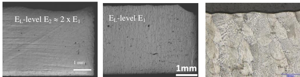
Figure 4: Micrographs for ODS-samples (left, middle) and etched IN625 sample (right)
