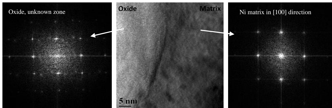
Figure 7: Microstructural analysis precipitates in IN625-ODS. E_L = E_1 .
