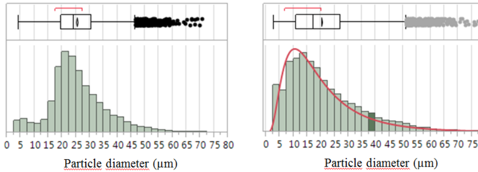
Figure 1: Particle size distribution of the IN625- (left) and IN625-ODS (right) powder. Furthermore, the powder can be distinguished in more detail using the Ellipticity E as the ratio of the major to the minor axis of a coextensive ellipse for each particle. The IN625 particles are more spherical with E = 1.25 \pm 0.26 , whereas the IN625-ODS particles are more elliptical ( E = 1.50 \pm 0.37 ) aligned with a higher shape variation and a more irregular particle surface, as shown in Figure 2 (middle and right).
