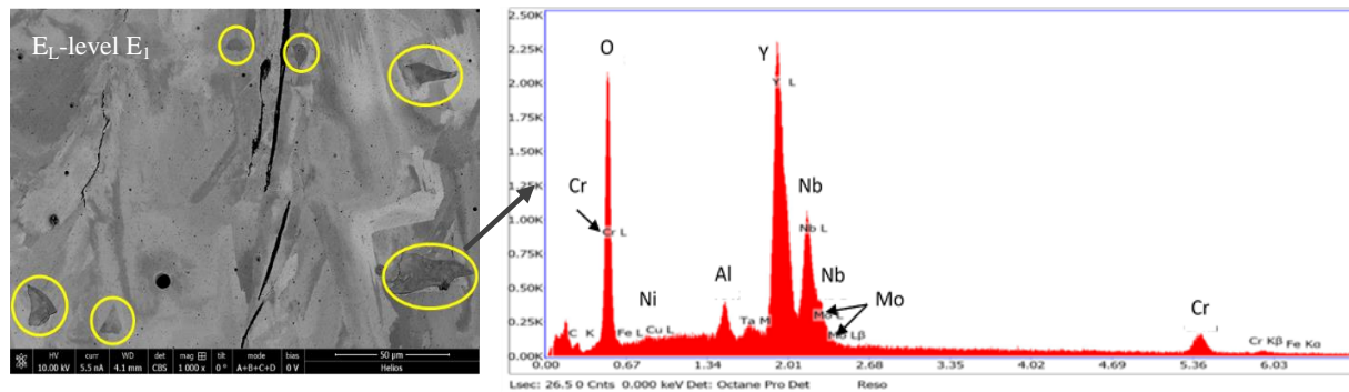
Figure 6: Top: Microstructural analysis of precipitates in IN625-ODS ( E_L = E_1 ), showing mainly signals of Nb, Cr, Y, Al, and O.
